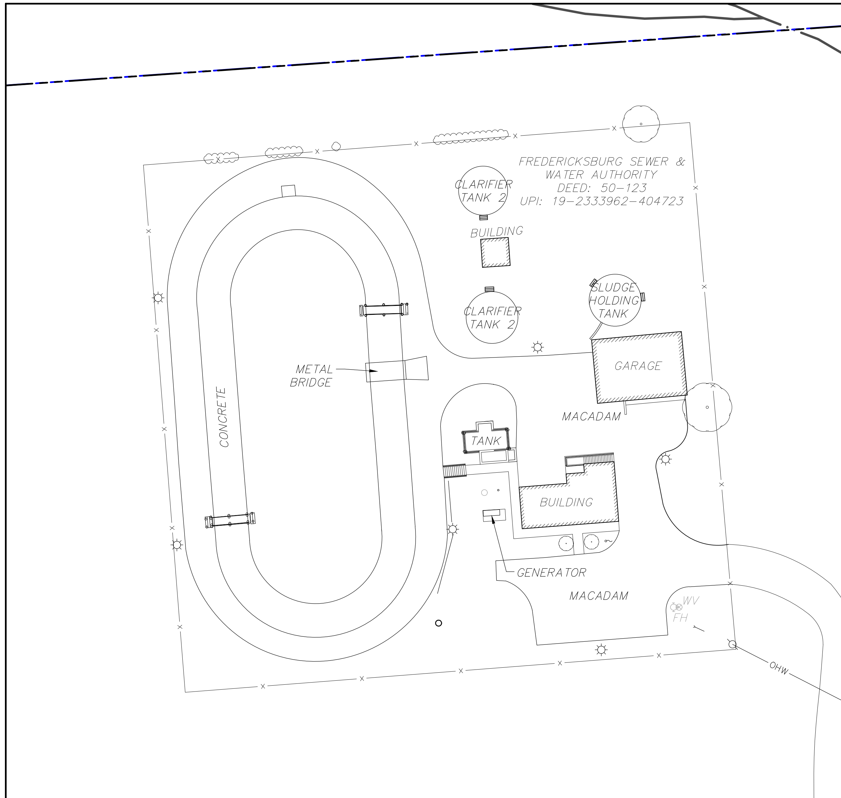
EXISTING CONDITIONS / DEMOLITION
